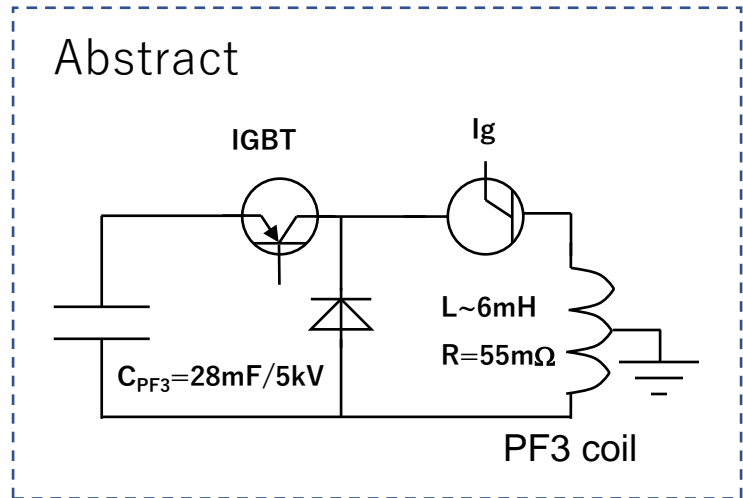
PF3 coil
